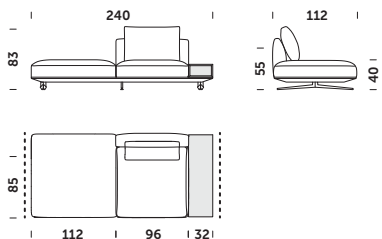
EOP_240 B 240x112x83cm
