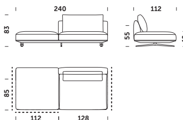
ENONP_240 A 240x112x83cm
