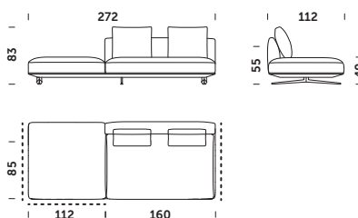
ENONP_272 A 272x112x83cm
